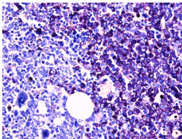
Figure 5. Bone marrow of the femur in Case 1. Mantle of neoplastic mast cells (central-right field) with cytoplasm containing Giemsa-positive granules replacing and comprising haematopoietic tissue. HE, 400x.
