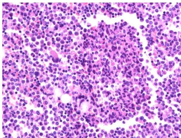
Figure 4. Bone marrow of the femur in Case 2. Hypercellularity, characterized by infiltration and partial replacement of haematopoietic tissue by dense groups of highly pleomorphic hypogranulated mast cells (central field). Hematoxylin and eosin staining. HE, 400x.
