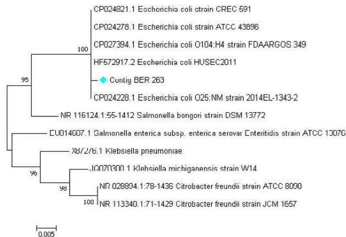
Figure 6. Molecular phylogenetic analysis by maximum likelihood method. The evolutionary history was inferred by using the maximum likelihood method based on the Tamura 3-parameter model [1] and the evolutionary analyses were conducted in MEGA7[2].
