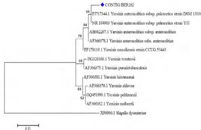
Figure 5. Molecular phylogenetic analysis by maximum likelihood method. The evolutionary history was inferred by using the maximum likelihood method based on the Kimura 2-parameter model [1] and the evolutionary analyses were conducted in MEGA7 [2].
